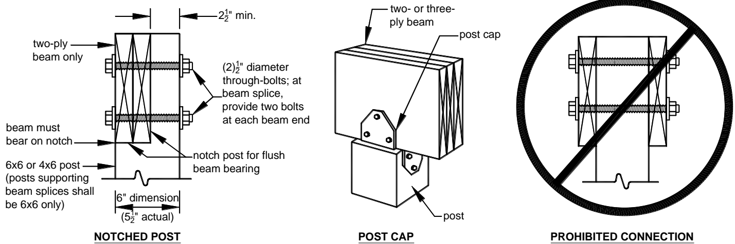
FIGURE 9: POST-TO-BEAM CONNECTIONS
