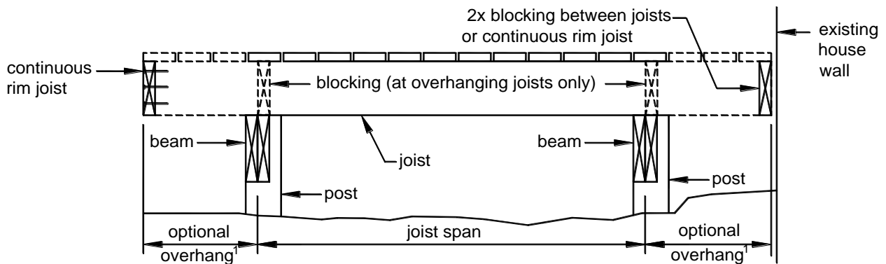
FIGURE 4: JOISTS WITH TWO DROPPED BEAMS/FREE-STANDING DECK (See Page 14 for more information.)
