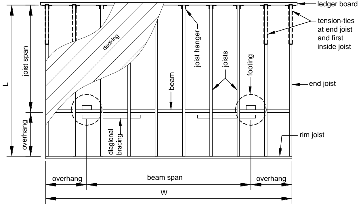
FIGURE 8: TYPICAL DECK FRAMING PLAN
