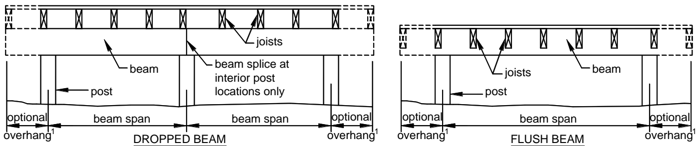
FIGURE 5: BEAM TYPES
