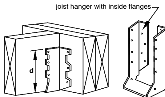
FIGURE 8: JOIST HANGERS
