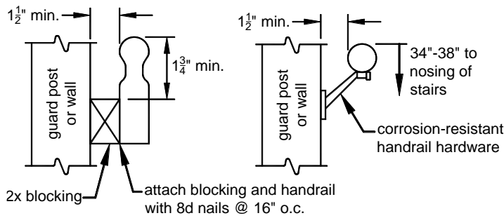
FIGURE 38: HANDRAILS
