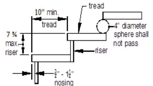
FIGURE 33: TREADS AND RISERS
